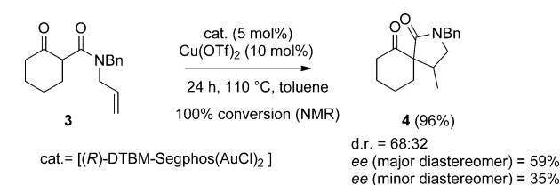
Scheme 1. Enantioselective hydroalkylation of an unactivated olefin.
